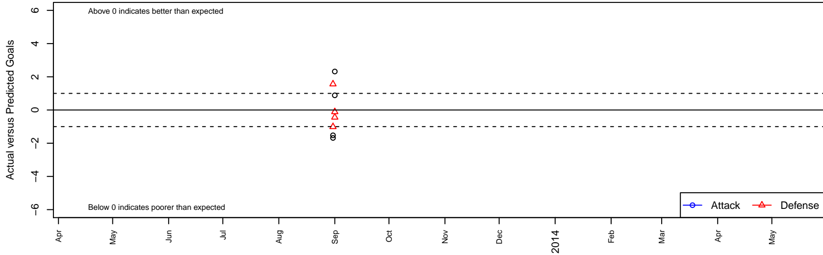
Monroe FC Cordova B95 Dots are actual minus expected GF (blue circles) and GA (red triangles). Blue line is smoothed change in attack strength. Red is smoothed change in defense strength.
